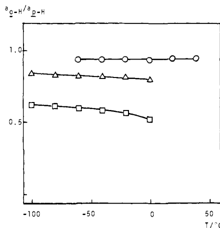
Figure 5. Temperature dependence of A o -H / A p -H . ○, 5; △, 3; □, 4.
