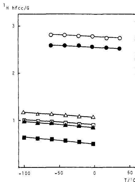
Figure 4. Temperature dependence of hfcc: ○, A p -H of 5; ●, A o -H of 5; △, A p -H of 3; ▲, A o -H of 3; □, A p -H of 4; ■, A o -H of 4.
